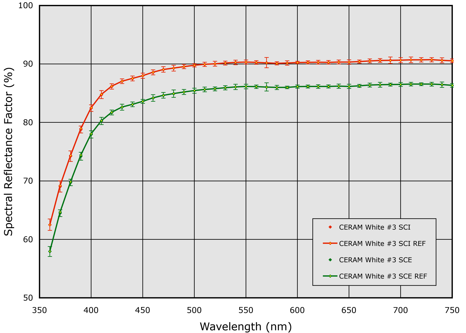
Reflectance Data for CERAM White Tile #3
