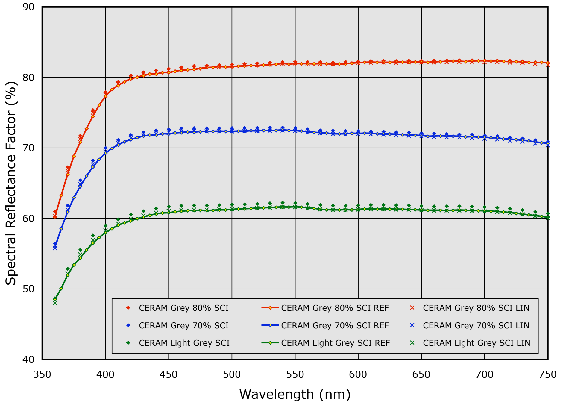
Reflectance Data for CERAM Light Grey Tiles
