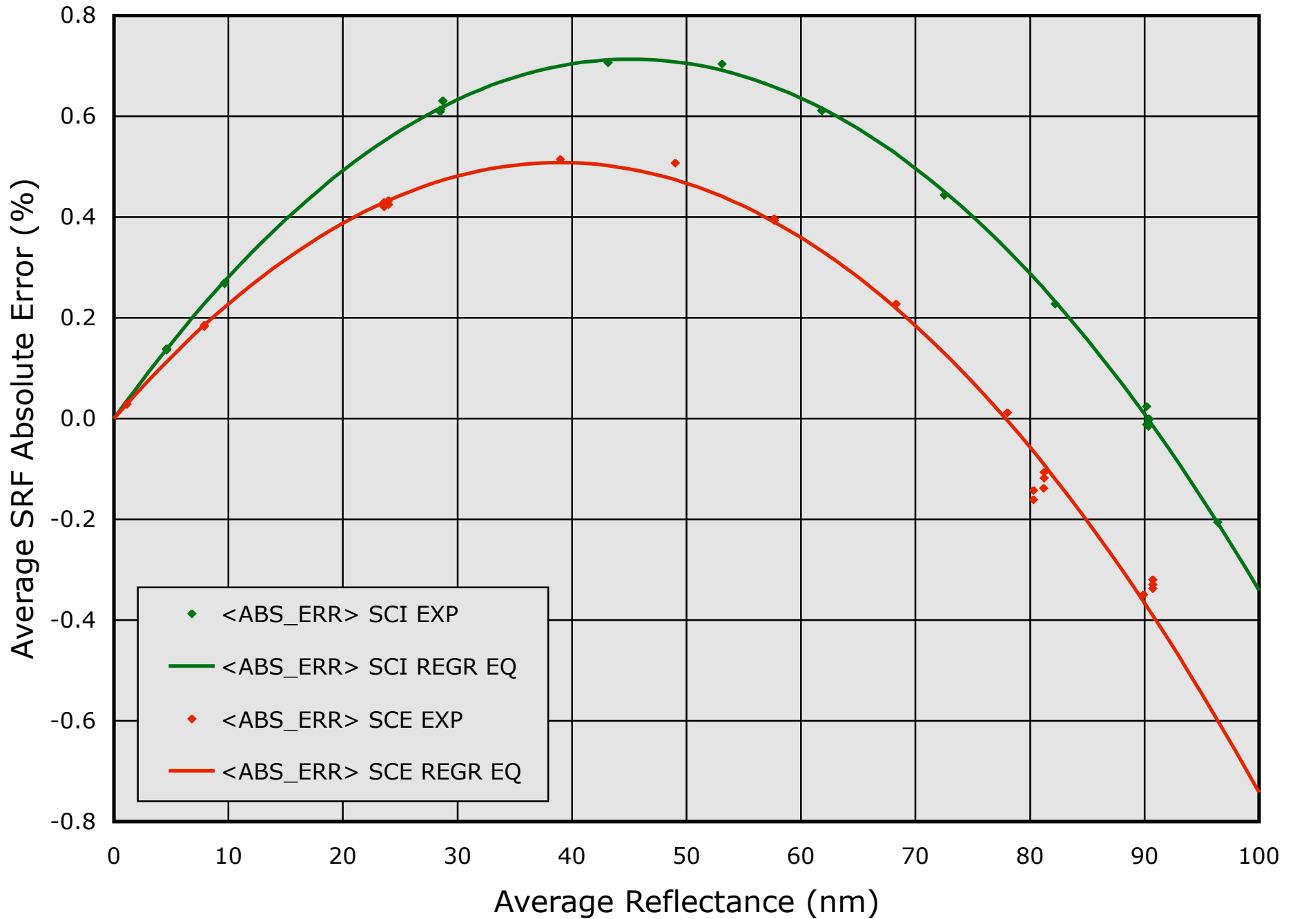
Nonlinear Photometric Scale for ColorEye 7000A vs. Lambda 19
