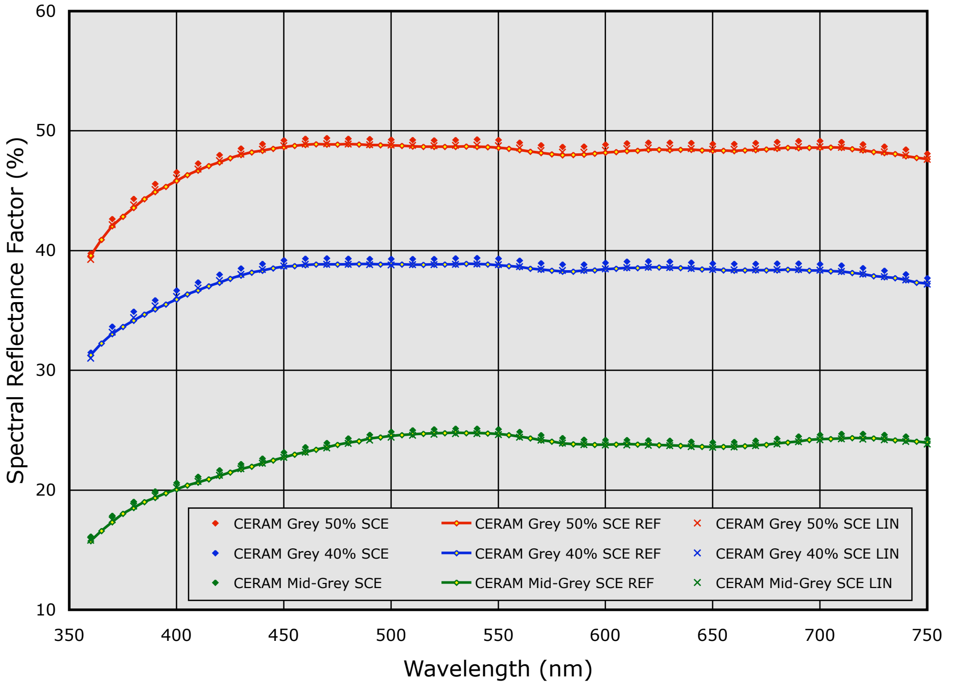
Reflectance Data for CERAM Medium Grey Tiles
