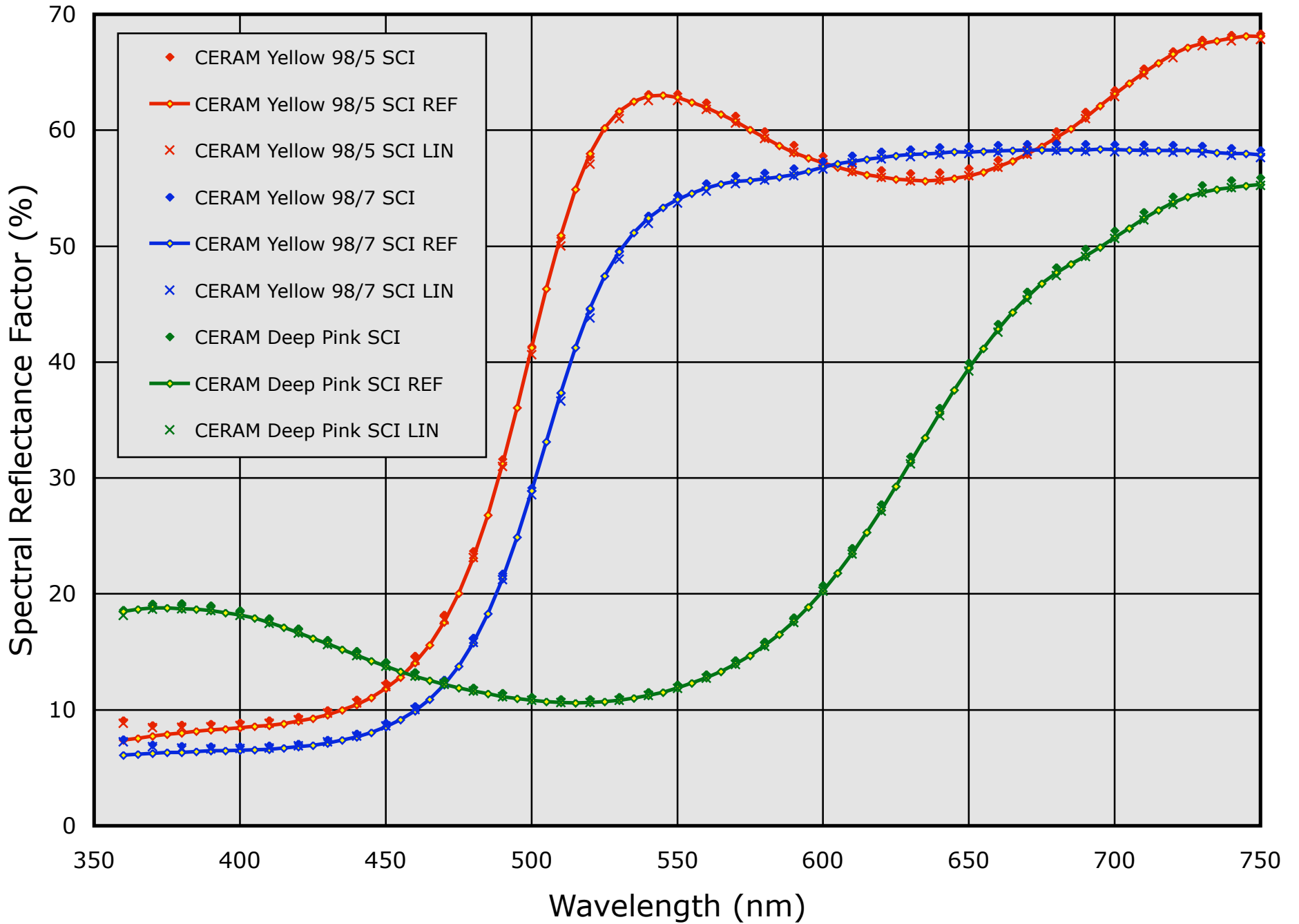
Reflectance Data for CERAM Chromatic Tiles
