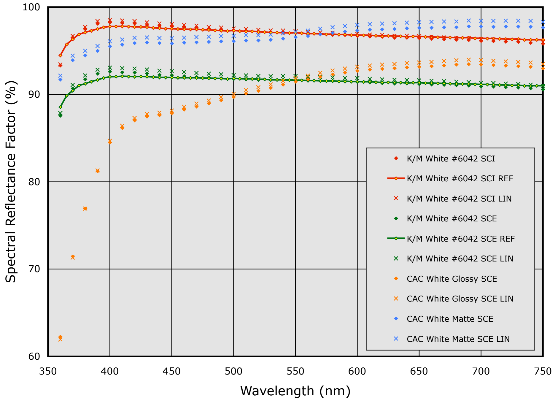
Reflectance Data for White Transfer Standards
