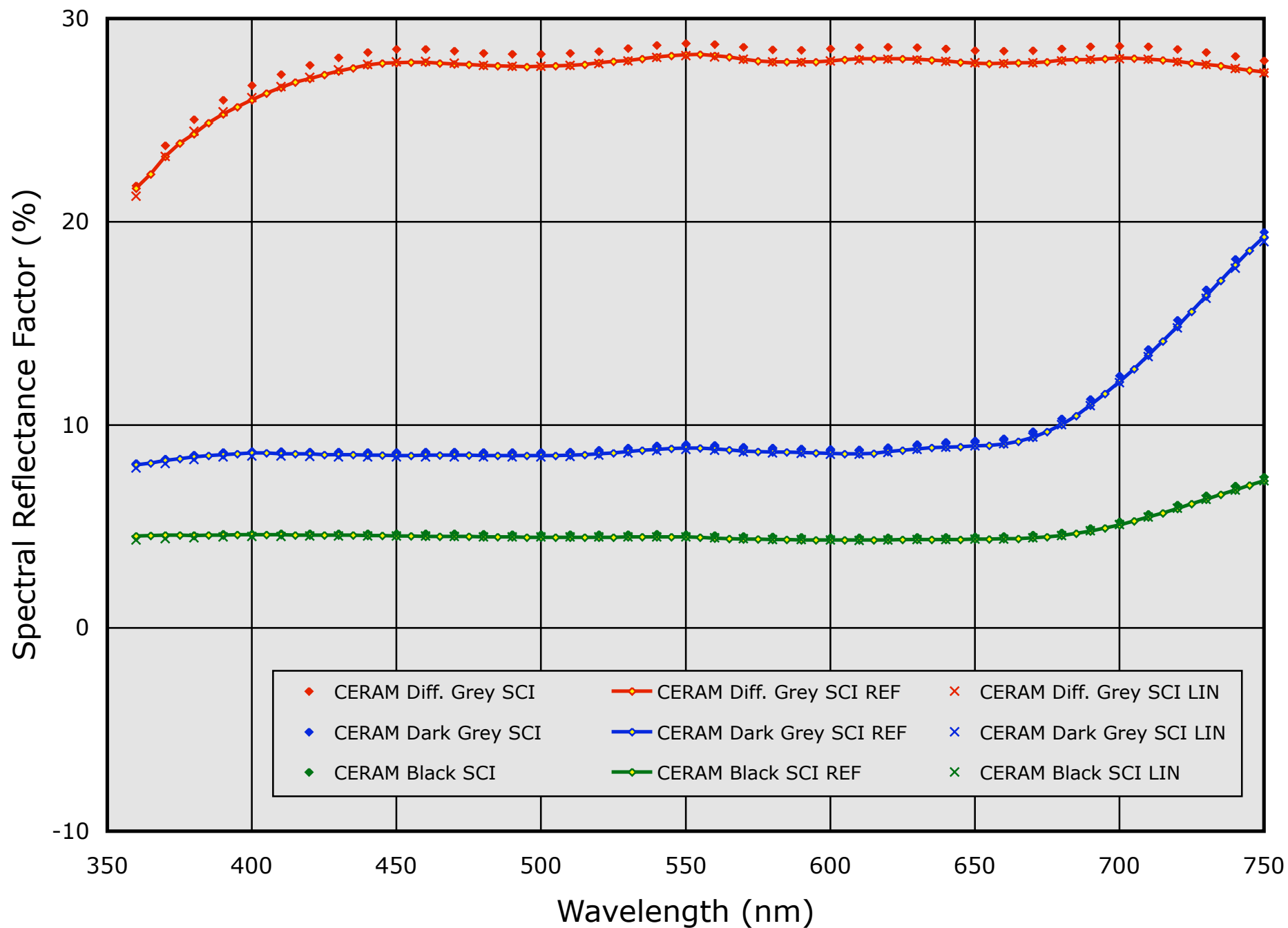
Reflectance Data for CERAM Dark Grey Tiles
