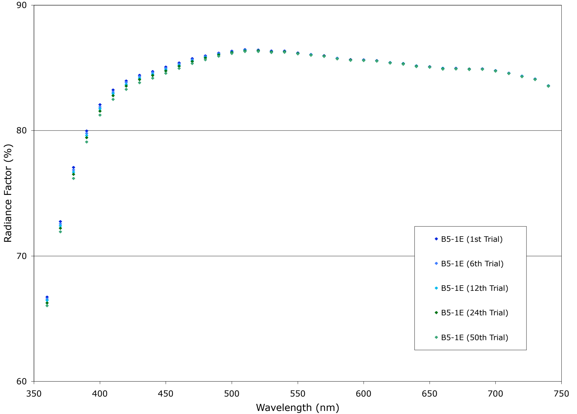
Systematic Loss of Reflectivity for B5-1 Tile with UV Exposure
