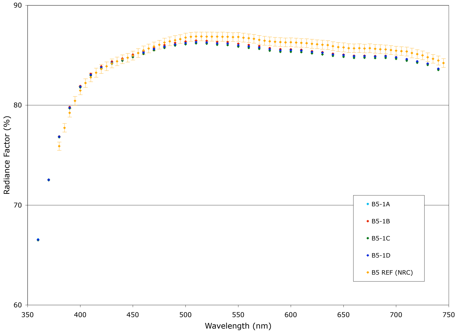
(45/0) Radiance Factors for Sectors A-D of B5-1 Tile
