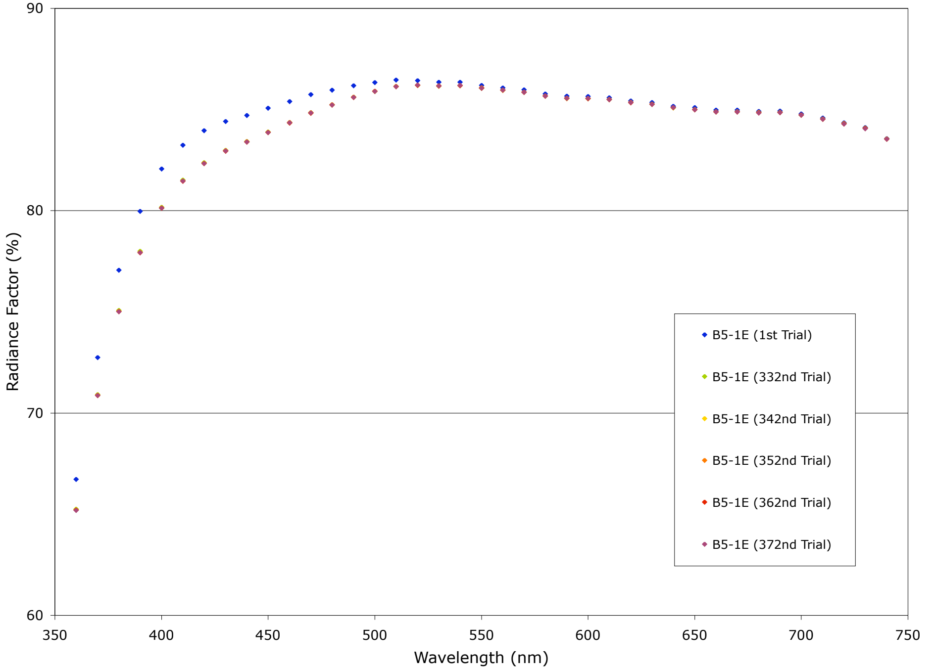
Saturation of Reflectivity Loss for B5-1 Tile with UV Exposure
