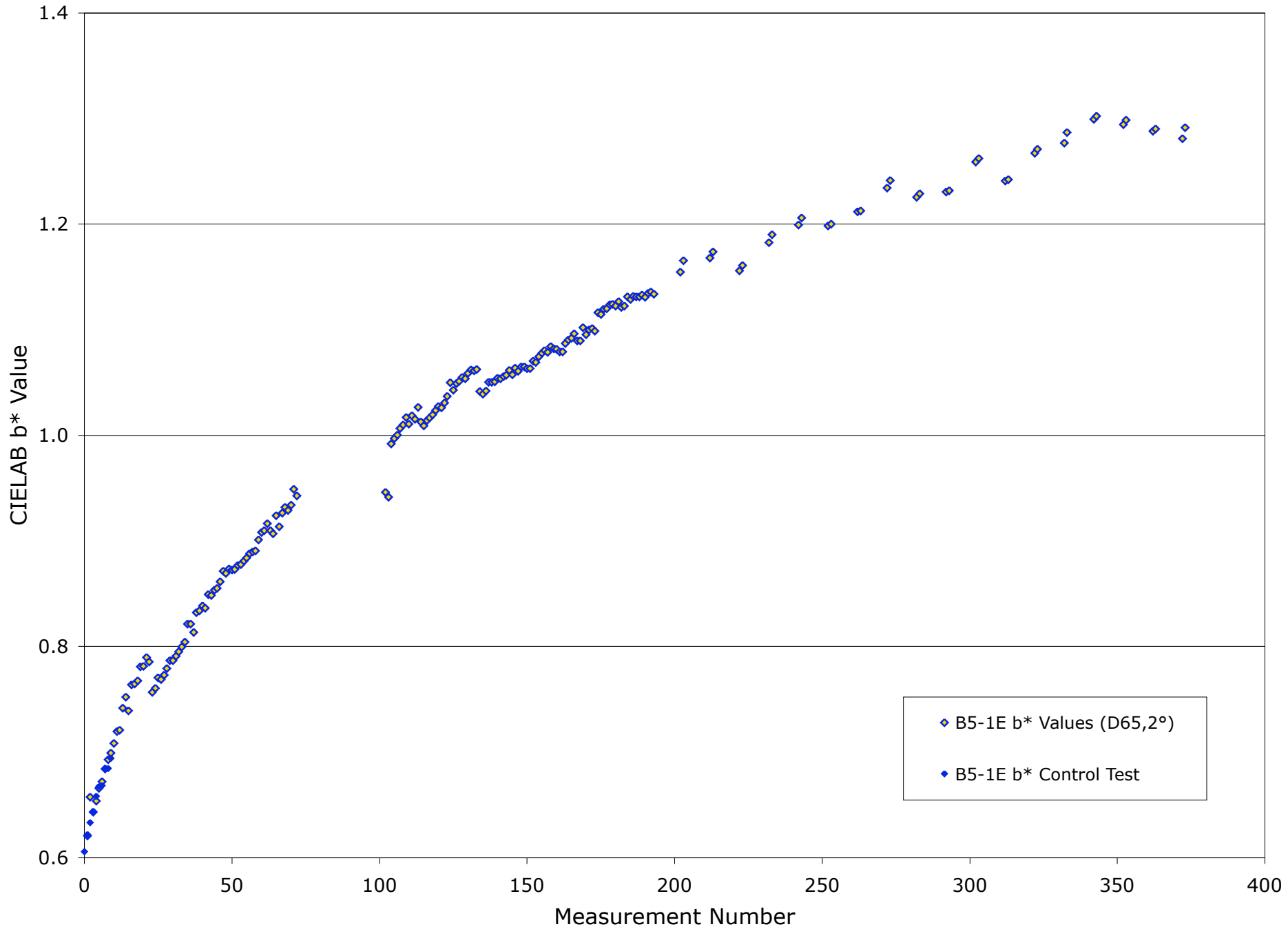
Change in CIELAB b* for B5-1 Tile with UV Exposure
