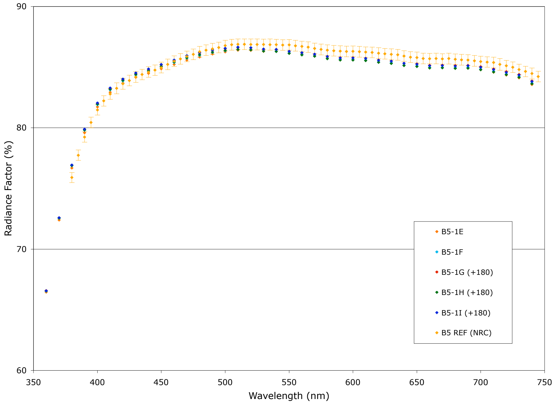
(45/0) Radiance Factors for Sectors E-I of B5-1 Tile
