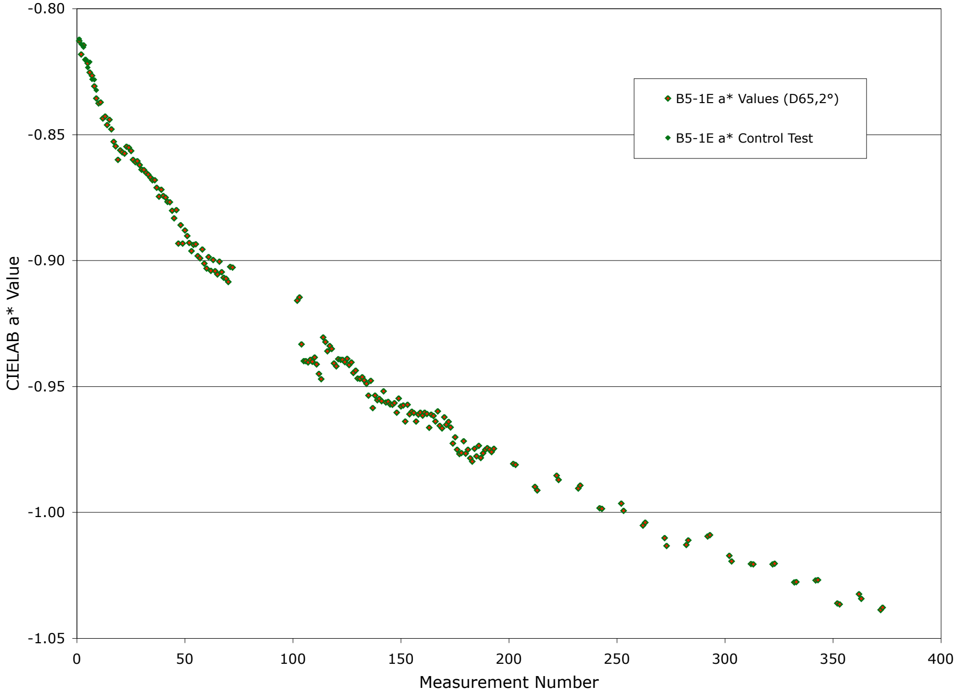
Change in CIELAB a* for B5-1 Tile with UV Exposure
