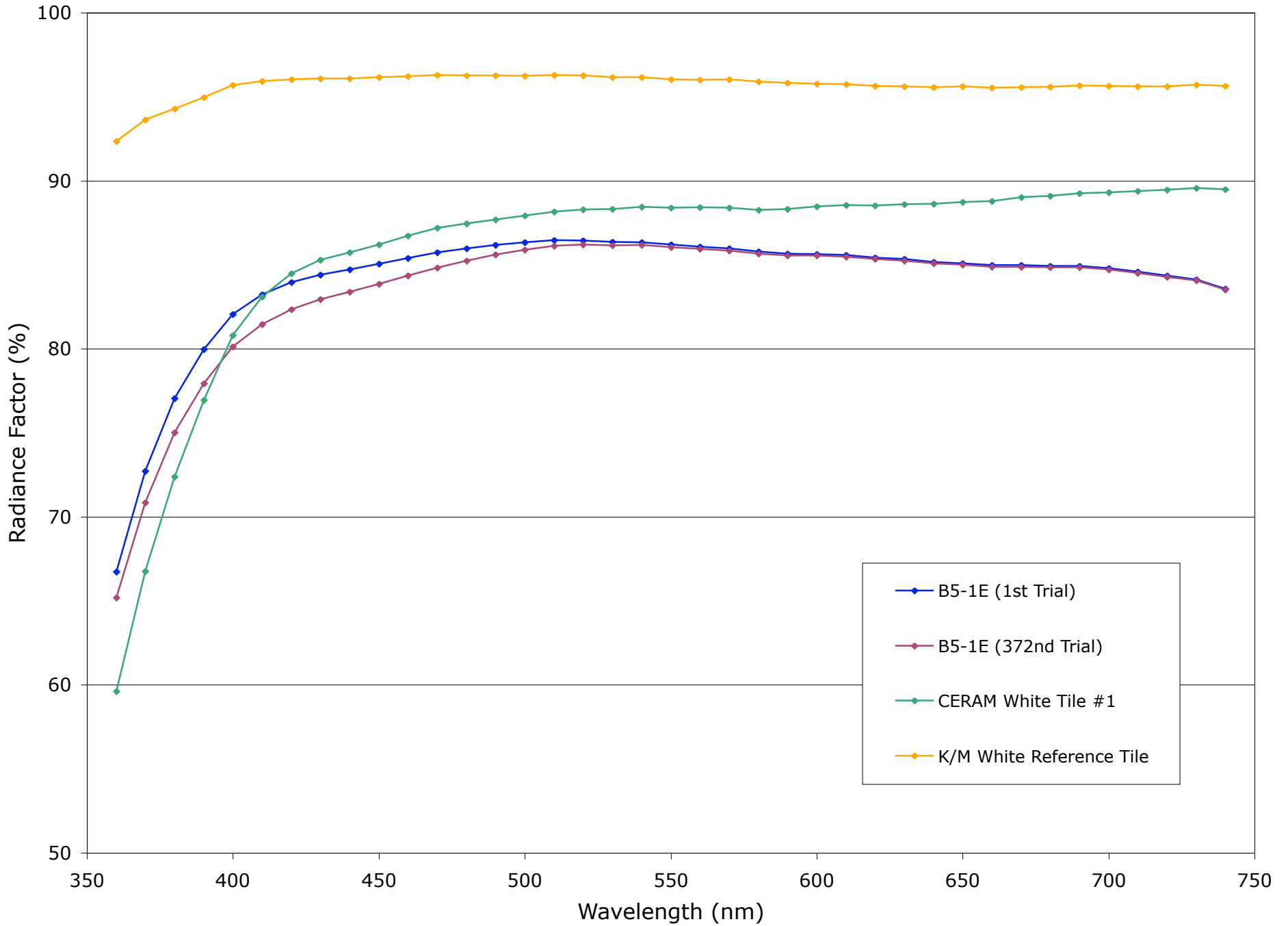
Comparison of UV-Exposed B5-1 Tile with Other White Standards
