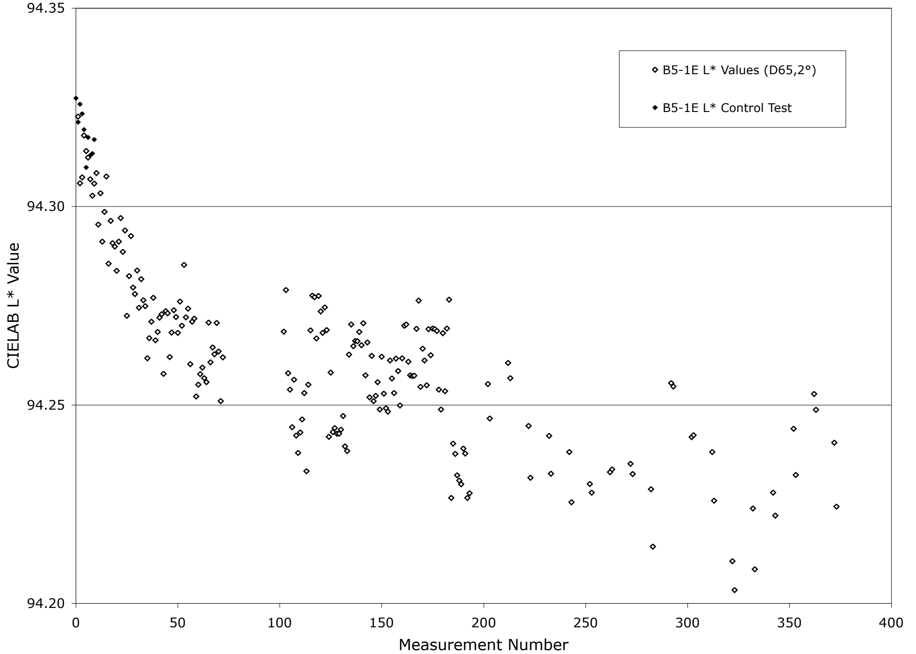
Change in CIELAB L* for B5-1 Tile with UV Exposure
