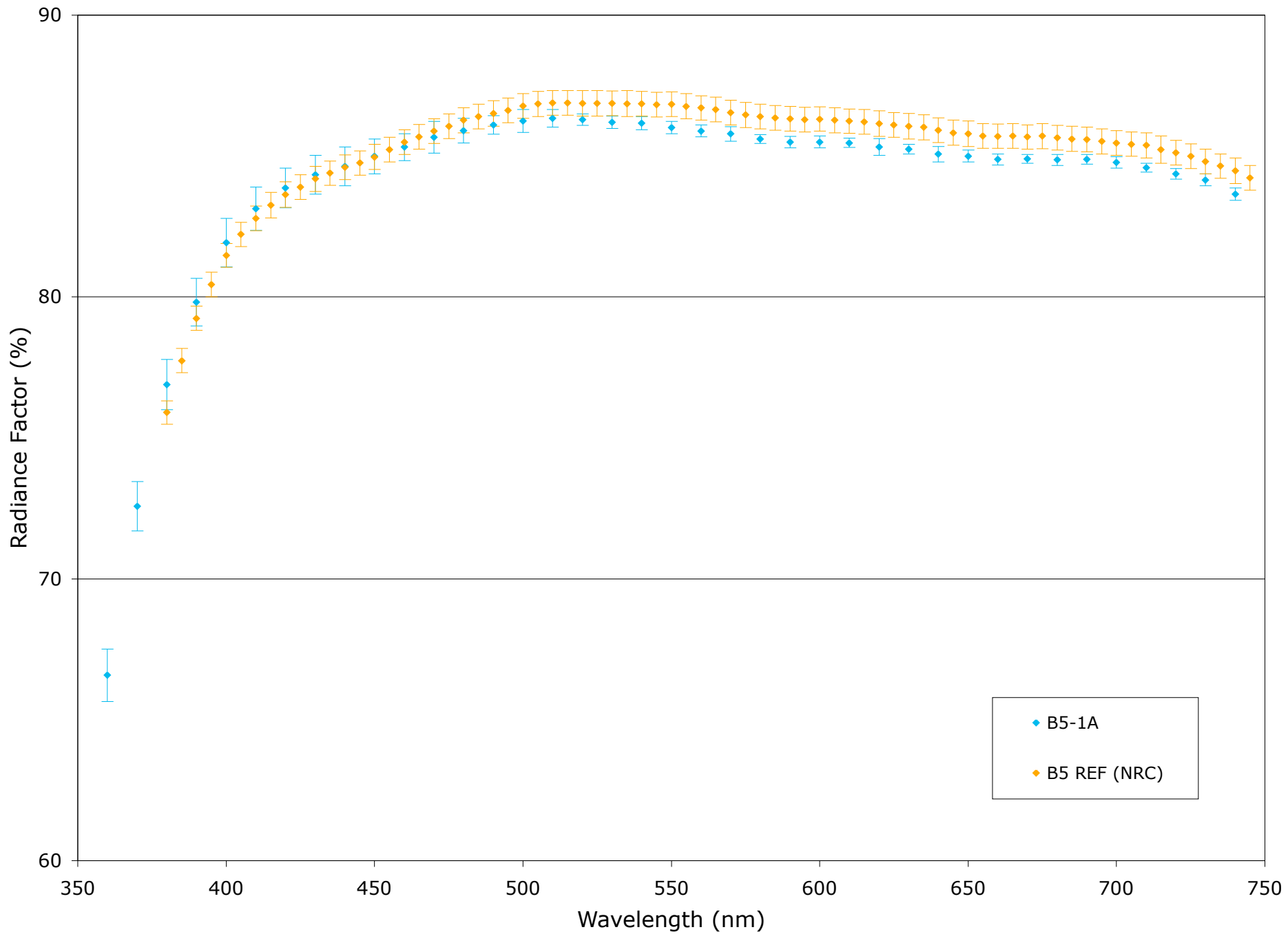
(45/0) Radiance Factors for Sector A of B5-1 Tile
